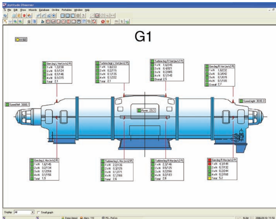
Example of a SKF @ptitude Observer process overview.
