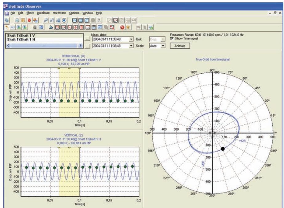
Example of a SKF @ptitude Observer orbit.
